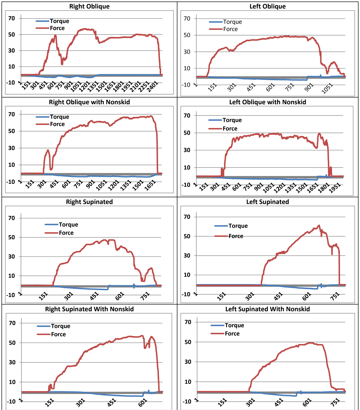
Supplemental Figure 1. Integral of the force (force-time) for a single force sensor and torque-time curves across all combinations of hand, approach, and nonskid material use. Every 150 units on the horizontal axis is equivalent to 0.3 s. Units on the vertical axis are Newton meters (Nm) for torque and N for force.
